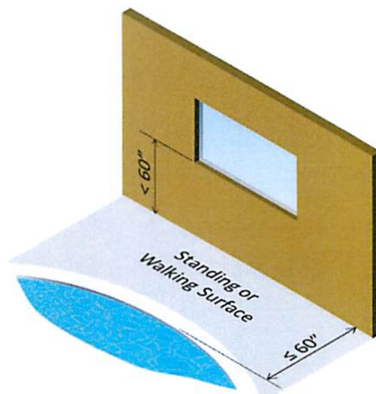
Figure 6 — Criteria for safety glazing adjacent to wet areas.
