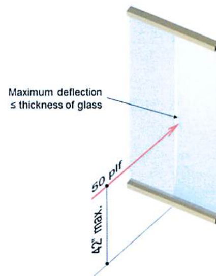
Figure 1 – Deflection of interior butt-glazed panels.
