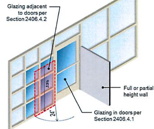
Figure 4 - Exception to requirement for safety glass when partition is between door and adjacent glass.
